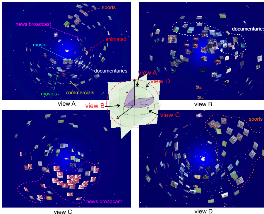
Fig. 2. Feature-based 3D movie representation (each movie is represented with one image). View A to D are screenshots made from different perspectives (the used points of view are synthesized with the system diagram presented in the center).
