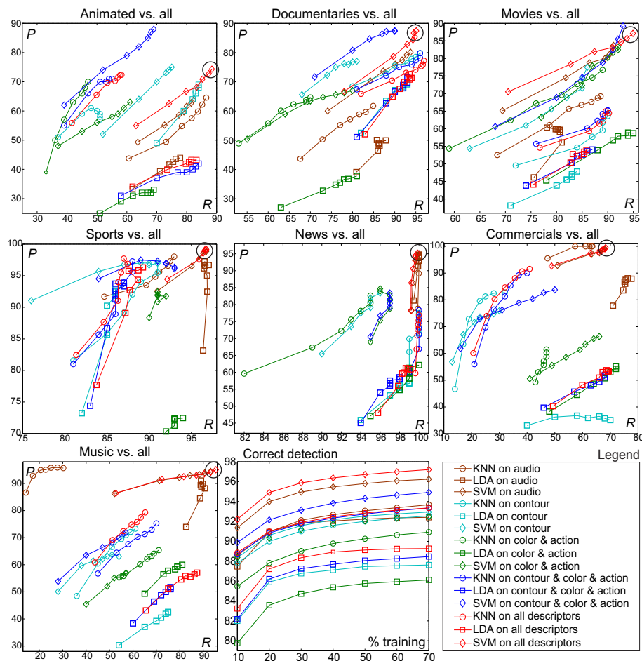
Fig. 1. Precision ( P ) against recall ( R ) for different runs and amounts of training data (increases along the curves from 10% to 70%) and overall correct classification ( \overline{CD} ).
