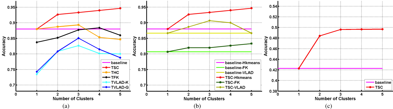
Fig. 1: Experiments on the Rochester ADL dataset: (a) the performance of different encoding approaches with a fixed BoW extraction method; (b) the performance when using a fixed encoding method (TSC) and different frame-based representations. The performance using the best pipeline on the Blip10k dataset is shown in (c). All the graphs are shown when the vocabulary size changes from 1 (no temporal variation) to 5 (highest temporal variation).
